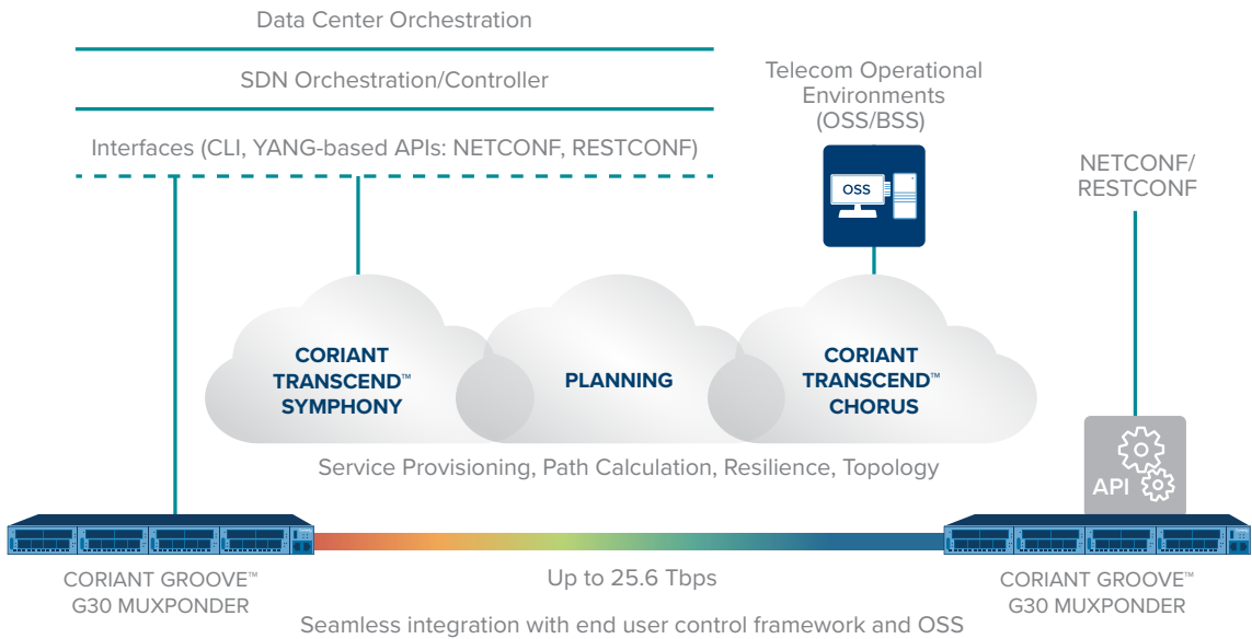
Figure 1: Coriant Groove™ G30 MUX Management and Control
